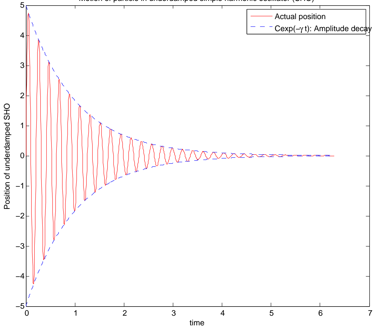
Motion of particle in underdamped simple harmonic oscillator (SHO)
