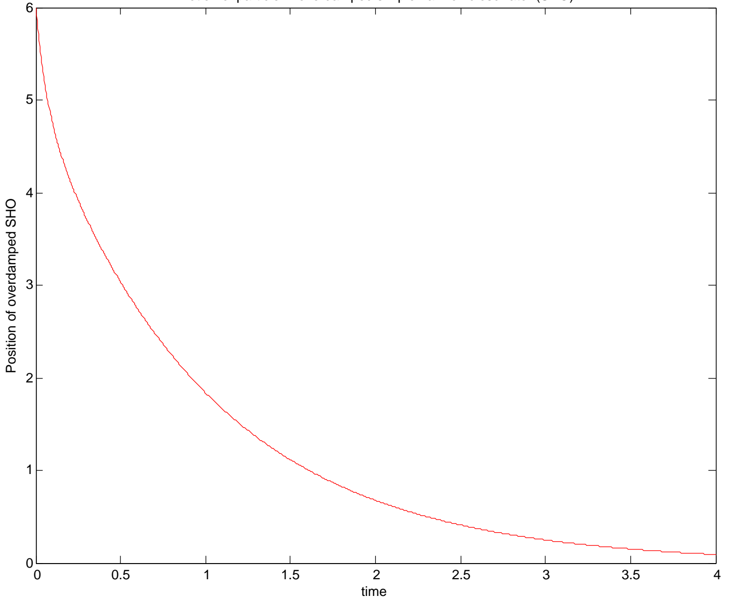
Motion of particle in overdamped simple harmonic oscillator (SHO)
